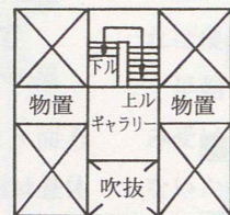
宿泊棟 3階
