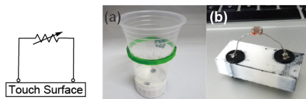
Figure 13. Tangible objects (a) with a thermistor (0.8 k \Omega –330 k \Omega ) and (b) with a CdS cell (10 k \Omega –1 M \Omega ).
