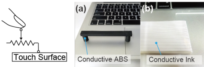
Figure 7. (a) 1-dimensional touch bar with conductive ABS (surface resistivity 10^3\Omega - 10^5\Omega/\text{sq} ); (b) 2-dimensional touch plate with conductive ink (surface resistivity 0.2\Omega/\text{sq} ).
